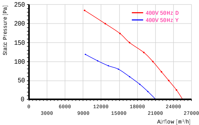
Airflow curve
