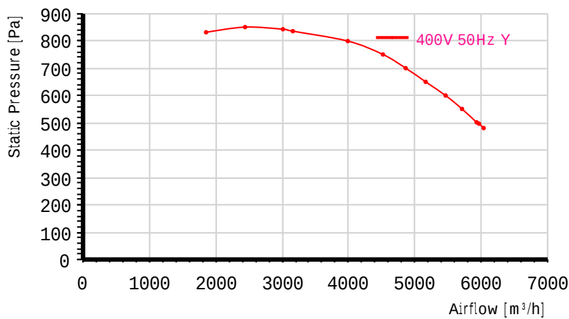
Airflow curve
