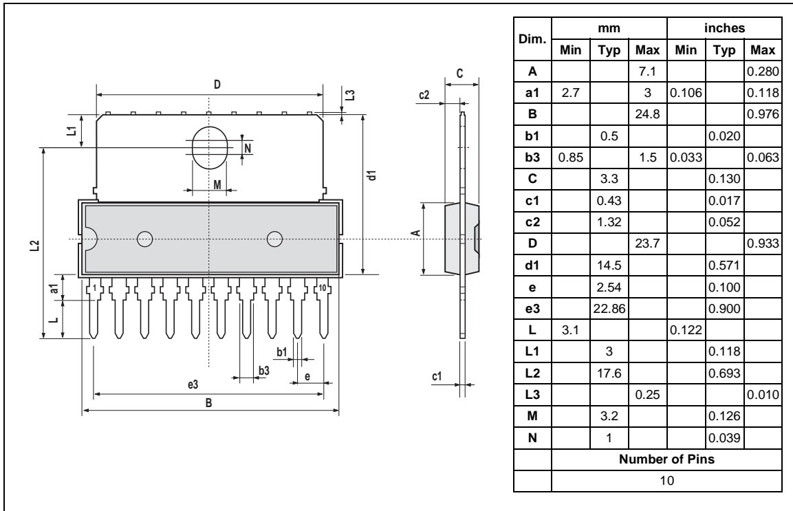
Figure 3. 10-Pin Plastic Single in Line Package
