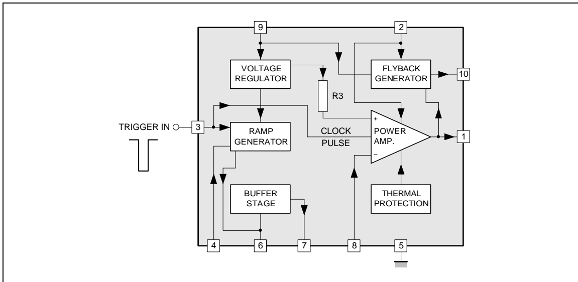
Figure 2. BLOCK DIAGRAM
