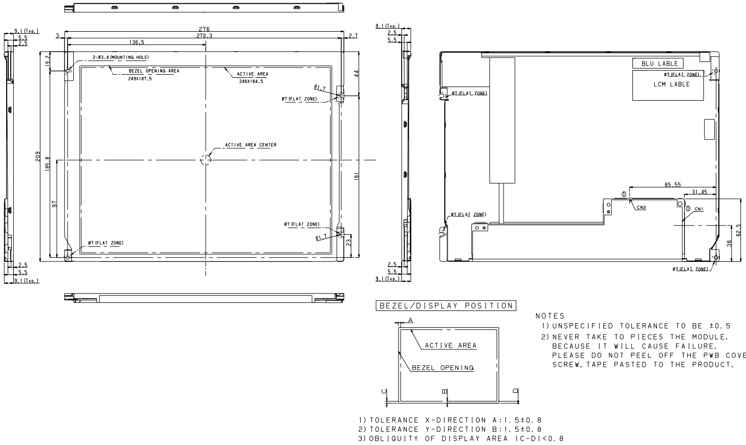
Fig.1 : LQ121S1LG88 OUTLINE DIMENSIONS
