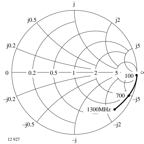
Figure 17. Output reflection coefficient
