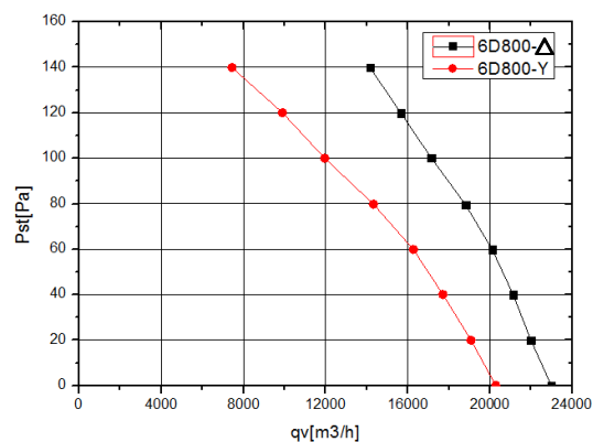
FLOW RATE CURVE (风量曲线) :
