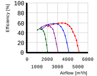
Efficiency on Static Pressure
