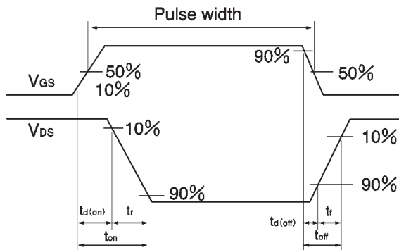
Fig.17 Switching time waveforms
