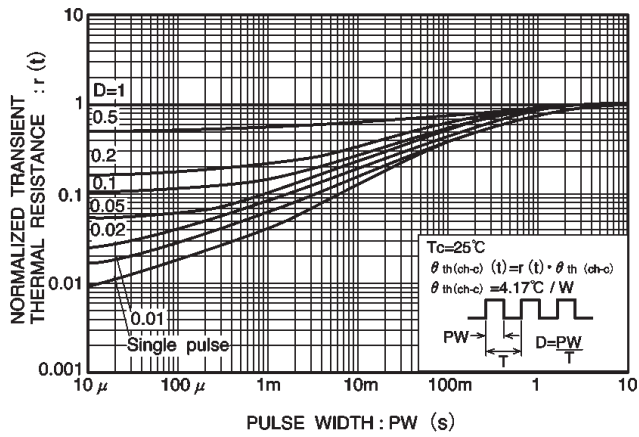
Fig.15 Normalized transient thermal resistance vs. pulse width
