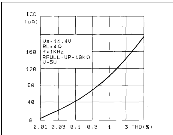
Figure 15. Clipping detector average current (pin 10) vs. distortion
