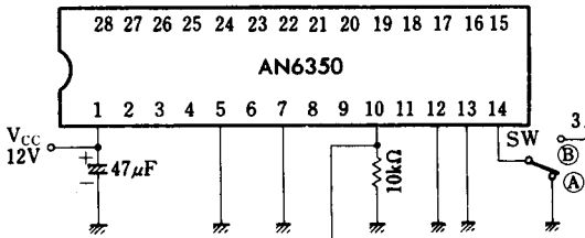
Test Circuit 10 ( V_{10} )
