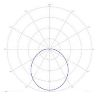
Cosmic LED 12W
