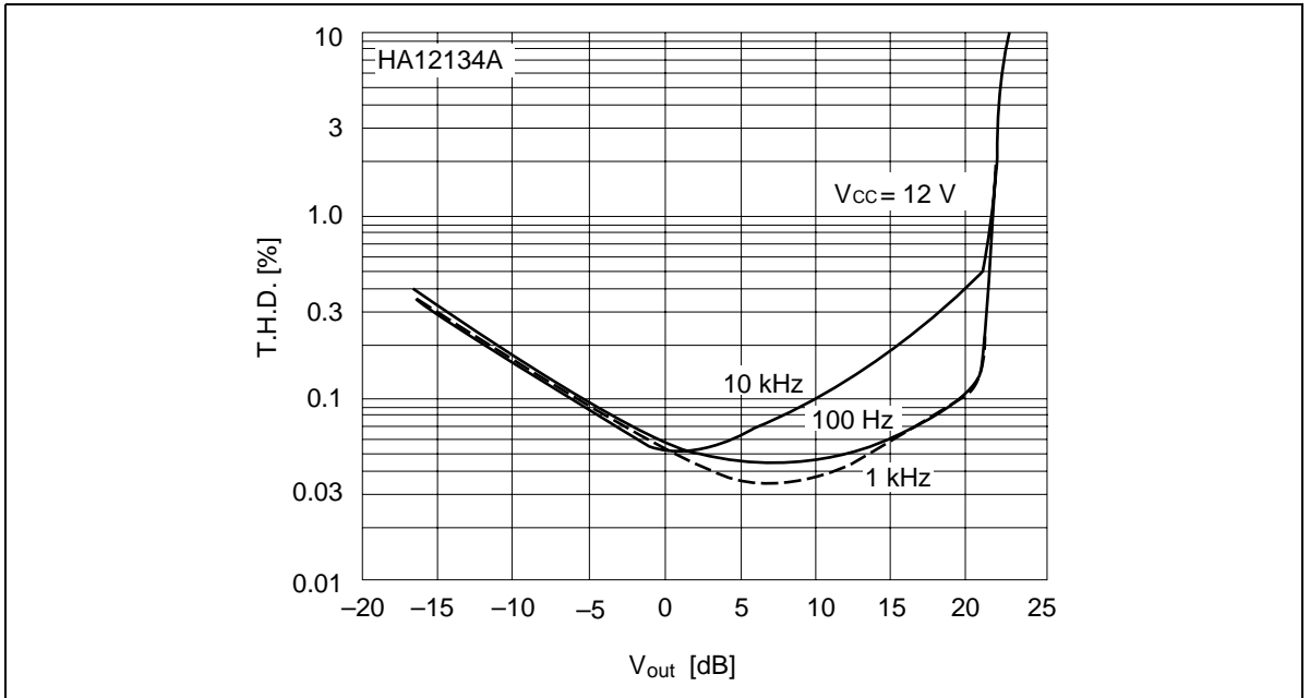
Figure 32 REC NR-ON Total Harmonic Distortion vs. Output Level
