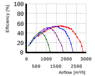
Efficiency on Static Pressure
