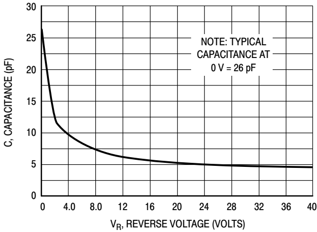
Figure 6. Typical Capacitance
