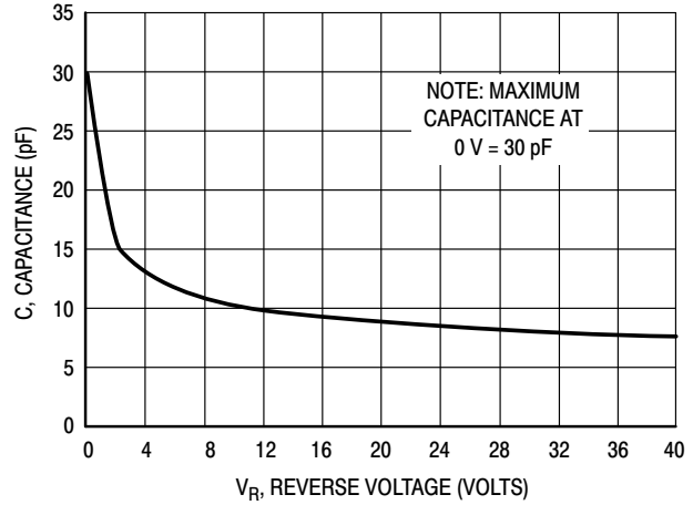
Figure 7. Maximum Capacitance
