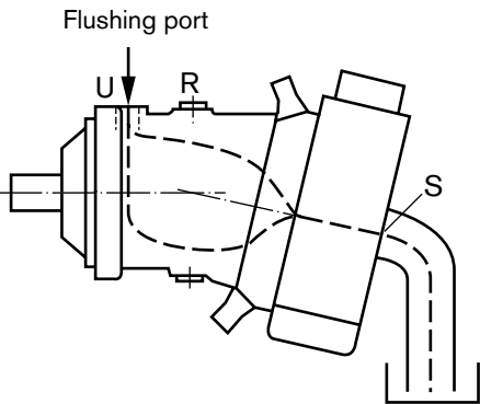
Flushing flows HA7VO (High-Speed-version)
