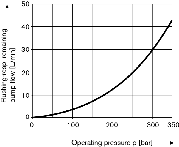
Flushing flows HA7VO (High-Speed-version)
