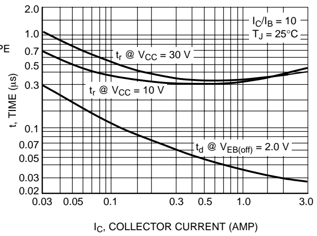
Figure 3. Turn-On Time
