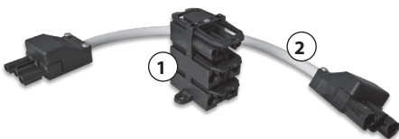
IR plug adaptor ① with cable ② - 94.2046 IR plug adaptor ① without cable - 94.4960
