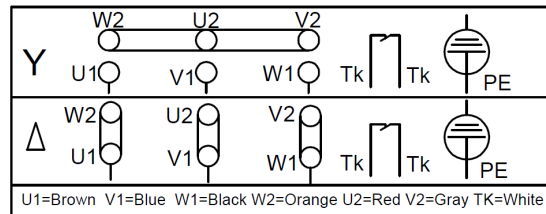
Wiring diagram(Default without thermal protector)
