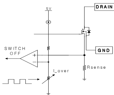
Figure 8. Soft Start Function
