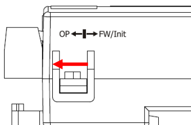
Figure 2-9 DIP switch (OP mode)
