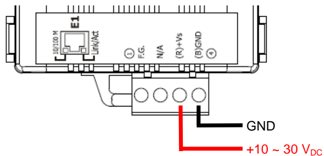
Figure 2-6 Power connection
