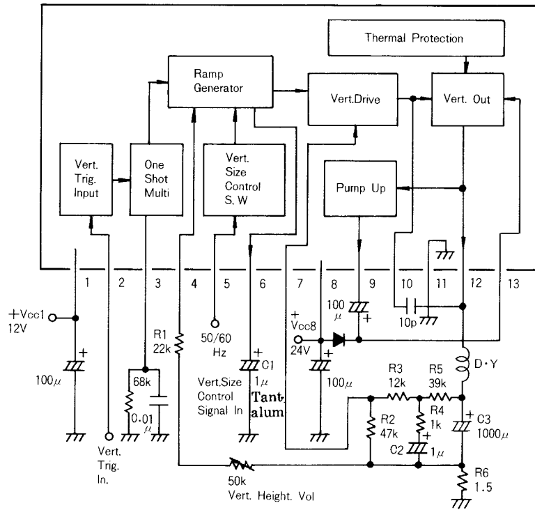
Fig. 1 +Vcc1, 12V
