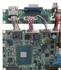
▲ Assembly view
