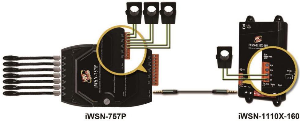
Fig.1. iWSN sensor and iWSN-757P connection diagram
