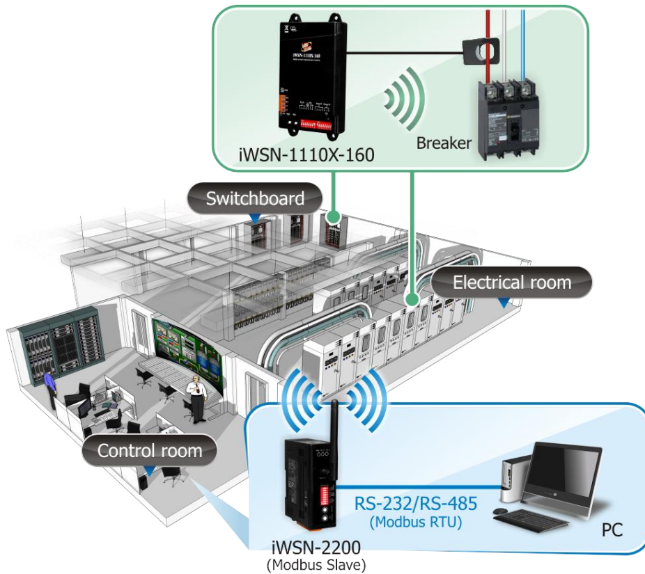
Fig.2. iWSN System application diagram
