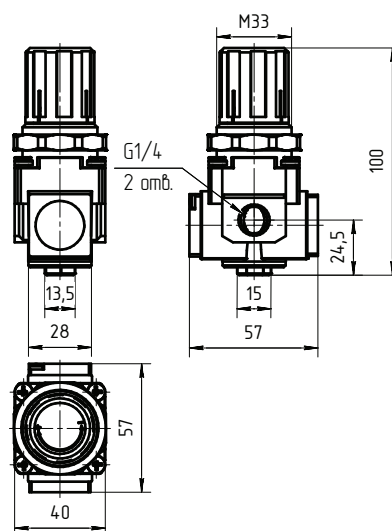
NXM2-1/4-R*0*
