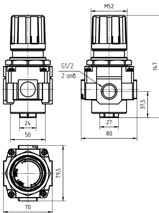
NXM4-1/2-R*0*
