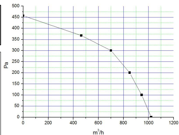
Airflow curves
