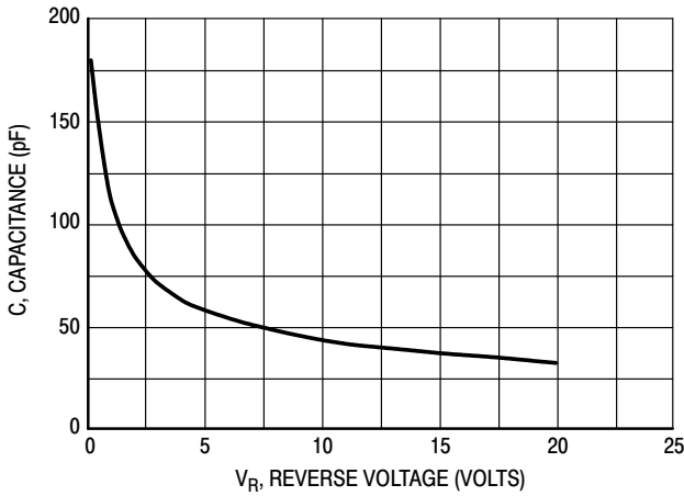
Figure 3. Typical Capacitance
