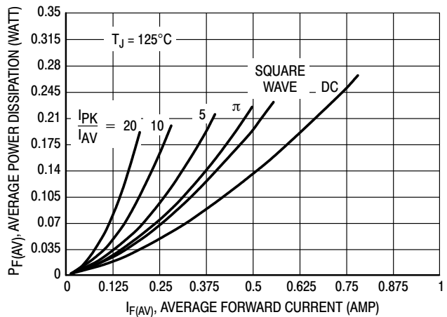
Figure 6. Power Dissipation
