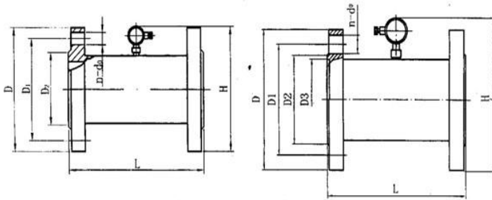
Flange connection structure
