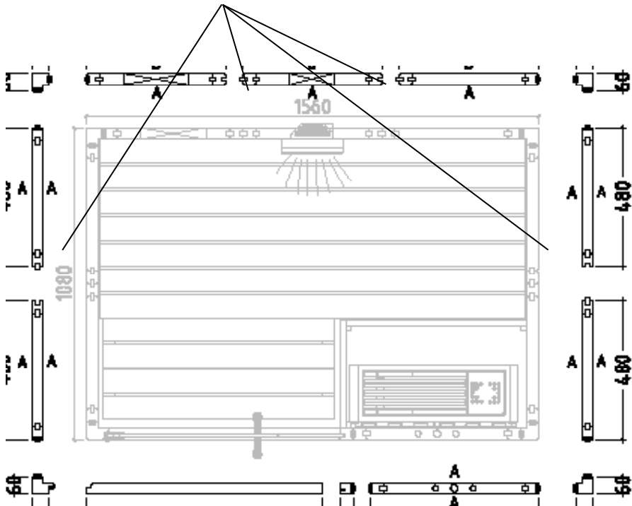
3 mm drill bit, 4 screws 4 x 70 mm
