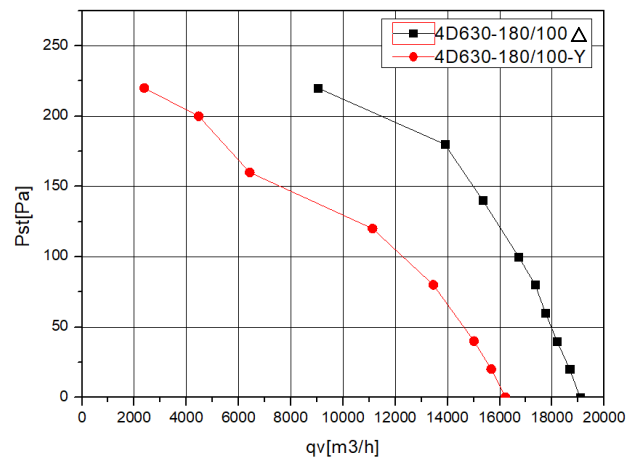
FLOW RATE CURVE (风量曲线):
