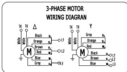
WIRING DIAGRAM (接线图):
