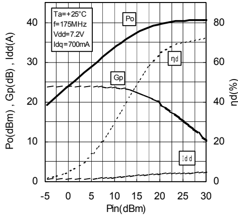
Pin-Po CHARACTERISTICS @f=175MHz
