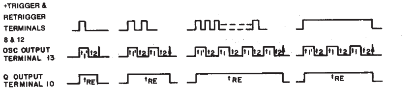
Fig. 34—Retrigger-mode waveforms.
