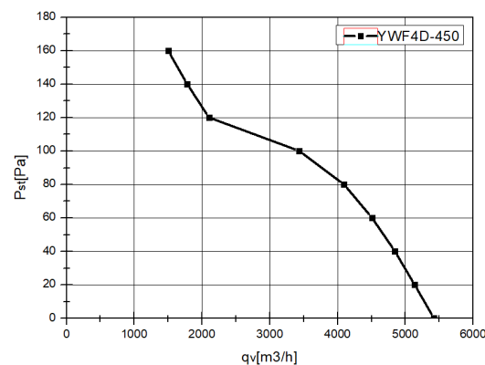
FLOW RATE CURVE (风量曲线) :
