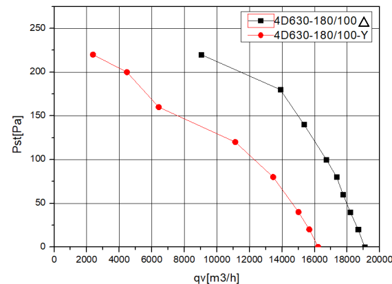
FLOW RATE CURVE (风量曲线) :
