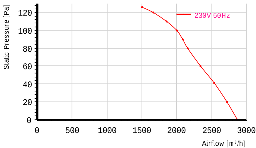
Airflow curve
