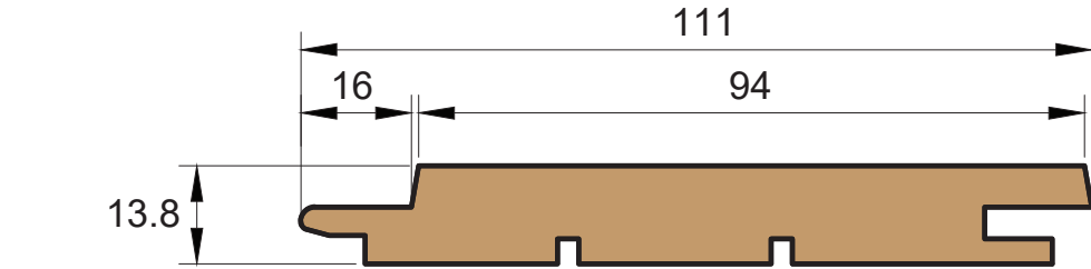
SIDE VIEW
