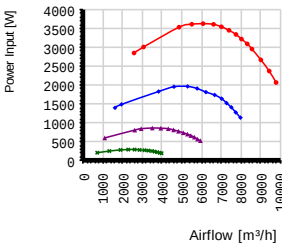
Power input
